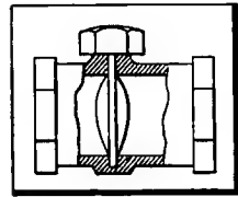
Fig. 1—Illustrating a common form of butterfly throttle valve. The valve is often punctured by a small hole so that the engine will just turn over when the valve is closed
